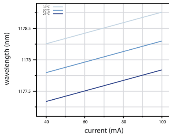
Fig. 2 Mode hop free tuning of 1178 nm based DFBs by current variation at different temperatures
