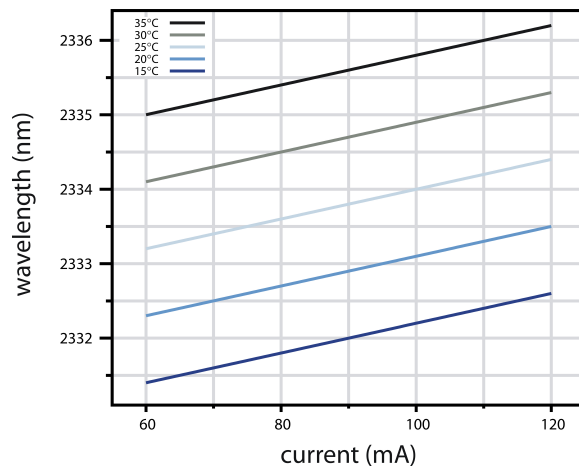
Fig. 2 Mode hop free tuning of 2334 nm based DFBs by current variation at different temperatures
