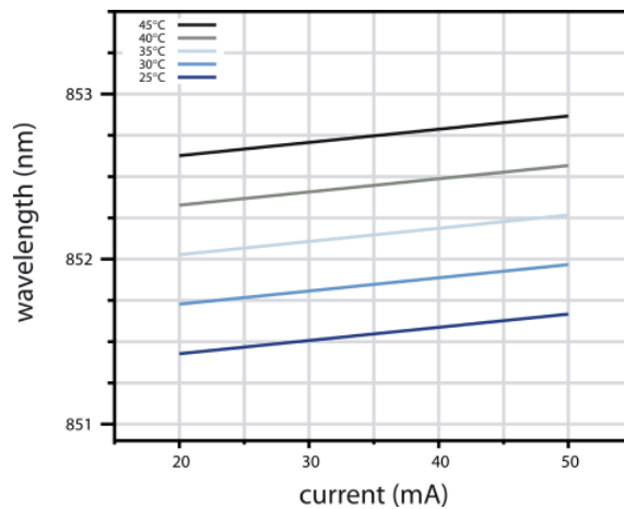
Fig. 2 Mode hop free tuning of 852 nm based DFBs by current variation at different temperatures
